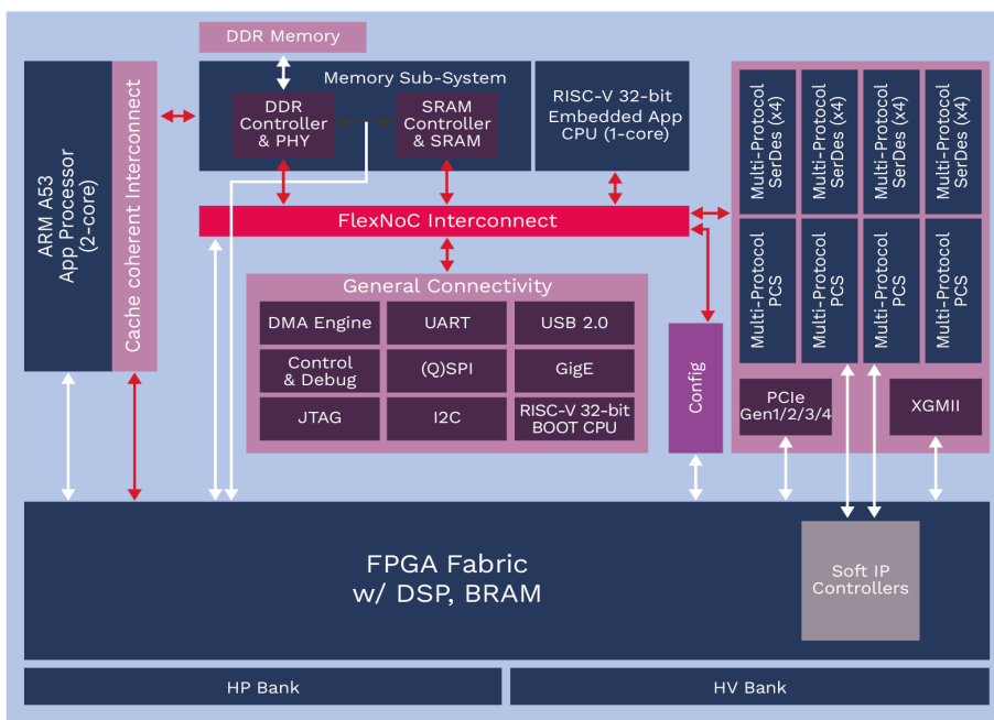
GEMINI BLOCK DIAGRAM
